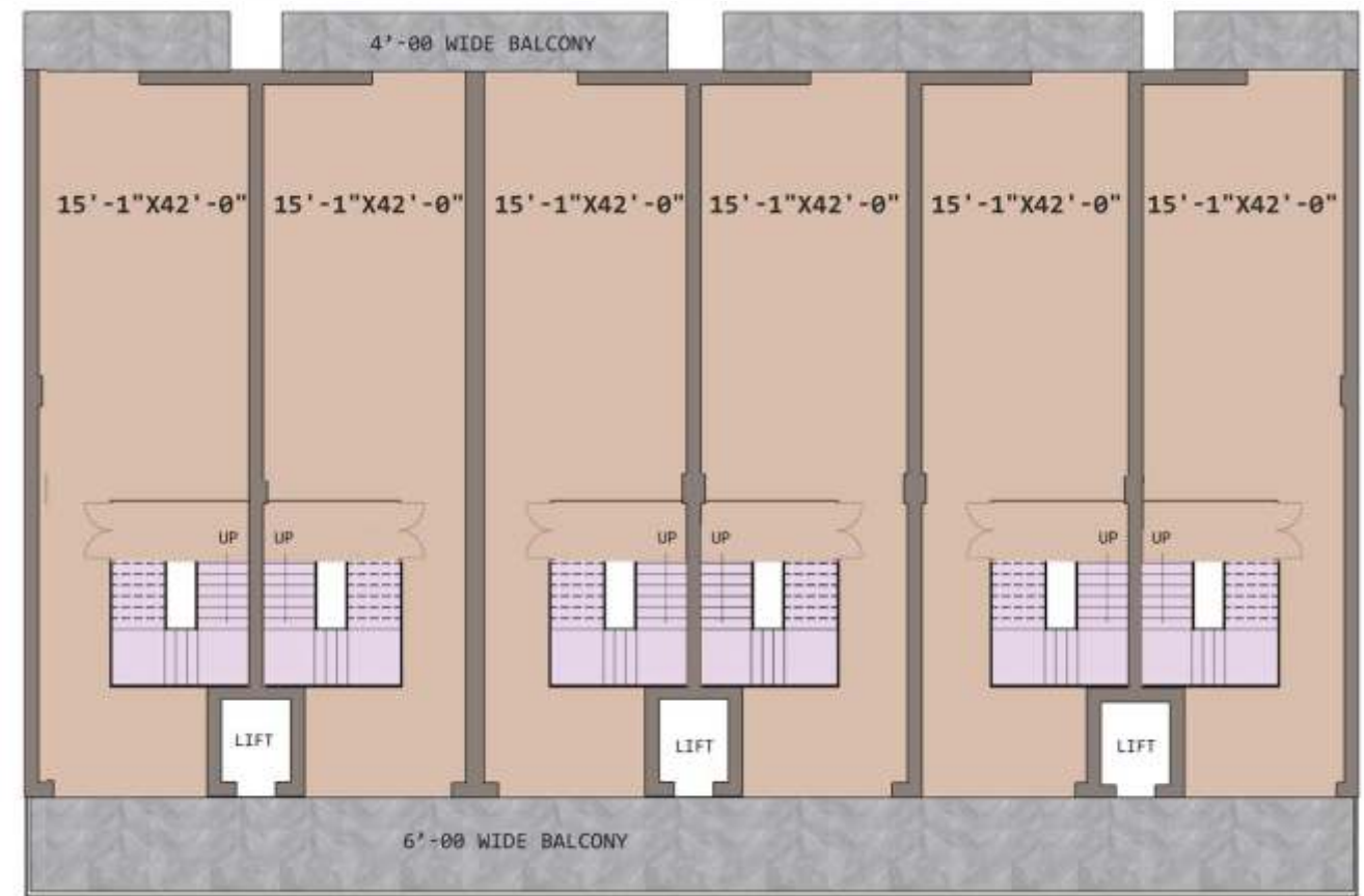
SECOND & THIRD FLOOR PLAN
